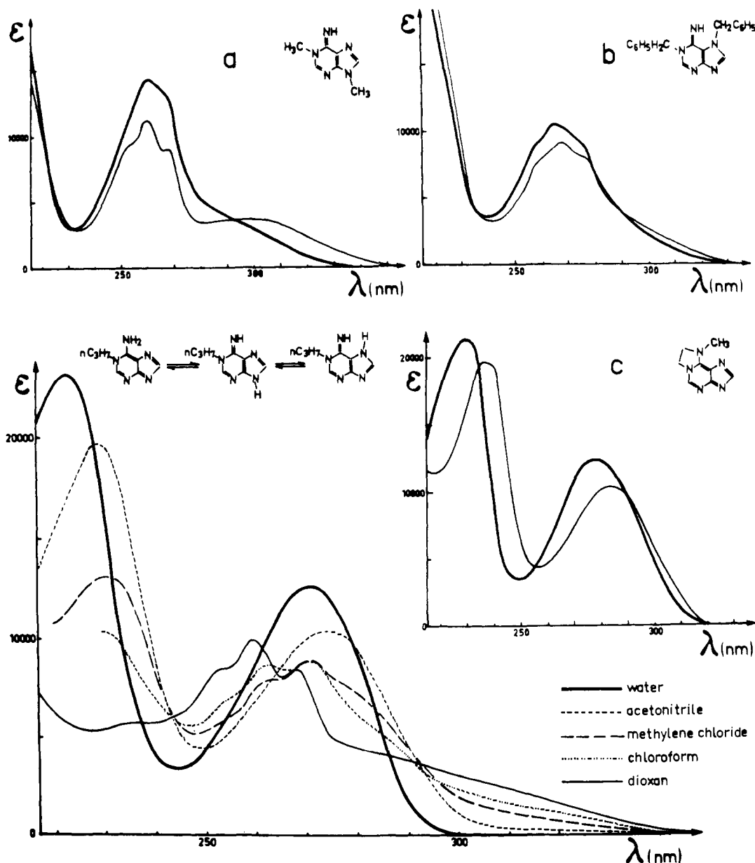
Figure 1. UV spectra of 1-propyladenine in different solvents compared with the spectra of nontautomerizable model compounds: (a) 1,9-dimethyladenine; (b) 1,7-dibenzyladenine; (c) compound IVb.
