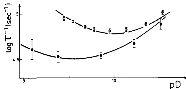
Figure 4. Plot of the relaxation times ( \tau ) observed with solutions of neutral 1-methyladenine in heavy water vs. pD (measured at the temperature before temp.-jump, t_i = 6 °C): 1-methyladenine concentration = 7.75 \times 10^{-3} M (upper curve) and 1.12 \times 10^{-3} M (lower curve); magnitude of the temperature jump = 6 °C; \lambda 300 nm.
