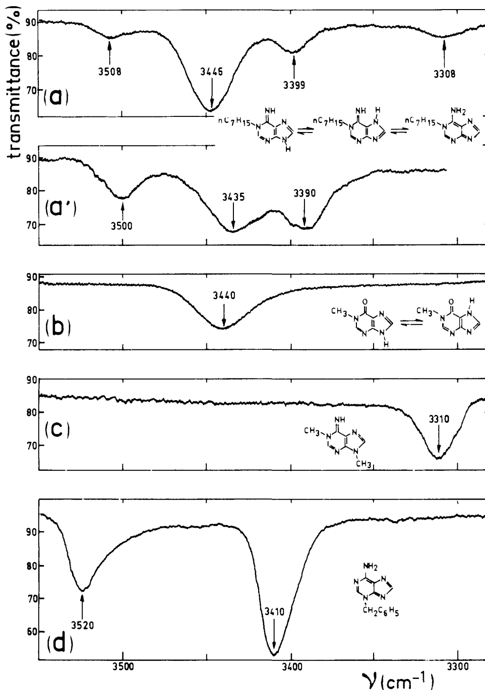
Figure 2. IR spectra in the NH stretch region of the following compounds (in chloroform solution unless otherwise stated): (a) 1-heptyladenine, 5 \times 10^{-4} M; (a') 1-heptyladenine, in methylene chloride solution; (b) 1-methylhypoxanthine, 2 \times 10^{-4} M; (c) 1,9-dimethyladenine, 2 \times 10^{-3} M; (d) 3-benzyladenine, 5 \times 10^{-4} M. All spectra were taken at 40 °C and using 2-cm optical length.
