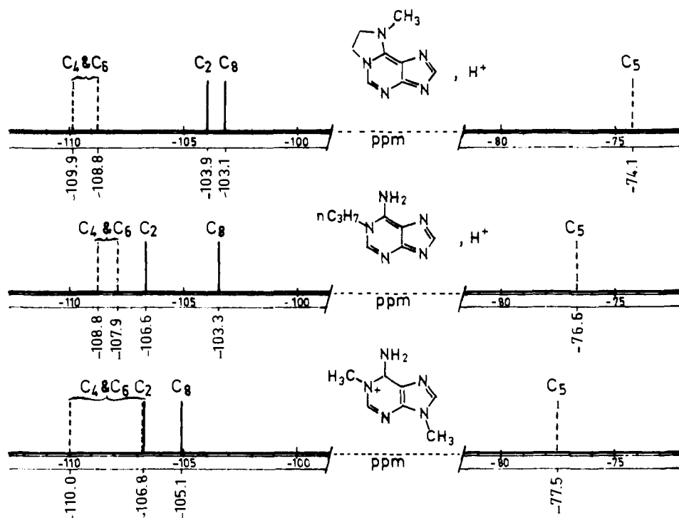
Figure 3. ^{13}\text{C} NMR spectra recorded in water for (from top to bottom) cationic IVb, cationic 1-propyladenine, and cationic 1,9-dimethyladenine (the aliphatic resonances are not shown). Chemical shifts are indicated in parts per million upfield from \text{Me}_2\text{SO} as an external reference. Dashed lines represent quaternary carbon resonances. The respective order of the \text{C}_2 and \text{C}_8 lines is in all cases inferred from that reported for the protonated adenine nucleotides. 38
