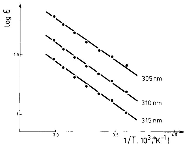
Figure 5. Plot of the 1-methyladenine extinction coefficient vs. (1/T) for different wavelengths; pD (as measured at 25 °C) = 8.6 (cf. text).
